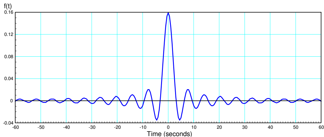
Impulse response of an ideal low-pas filter with a cut-of at 1 rad/sec
